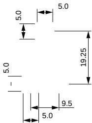
Land Pattern: [mm]
